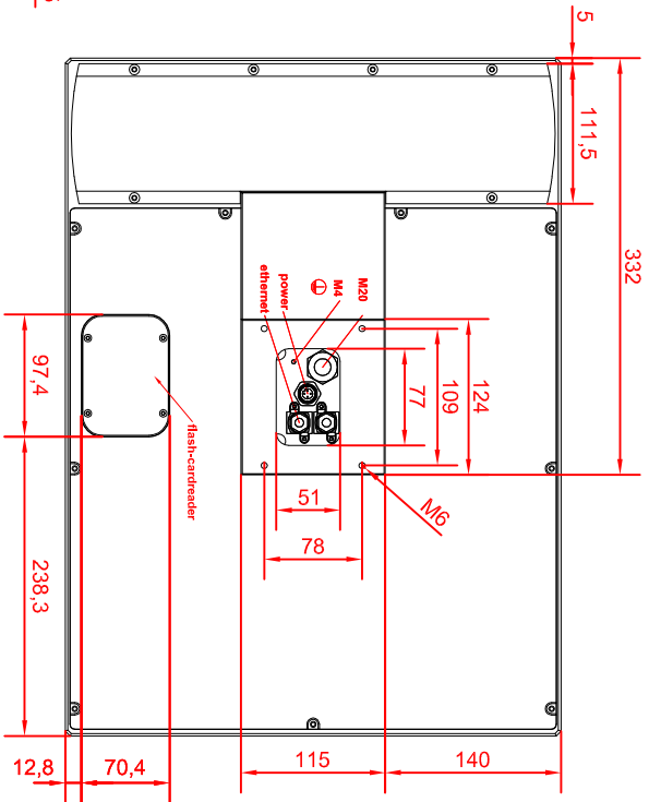
rear view
