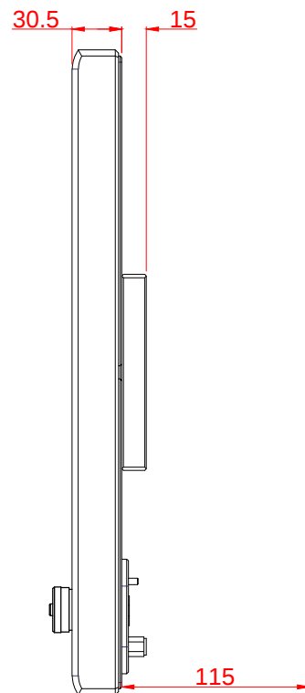
left view
