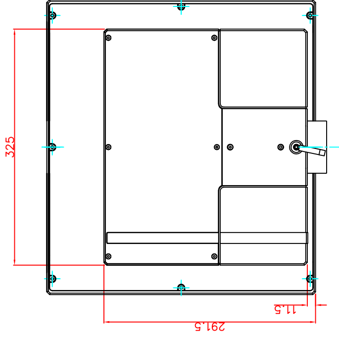
rear view
