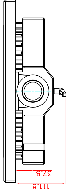
top view
