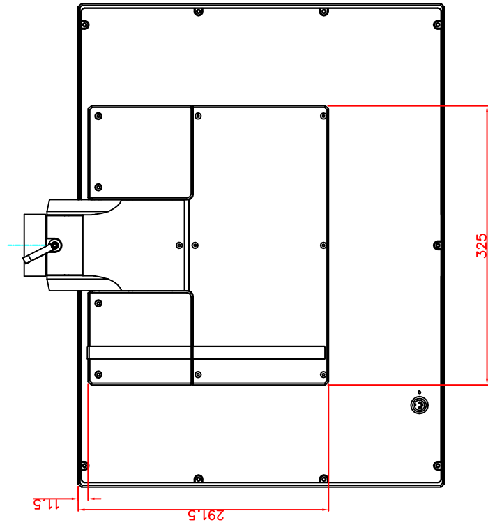
rear view
