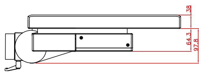
left view
