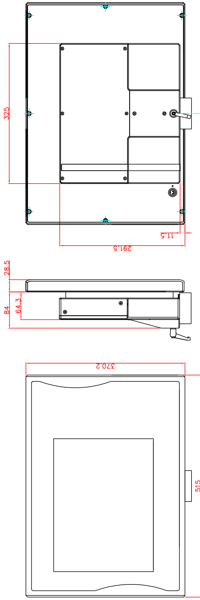
front view
