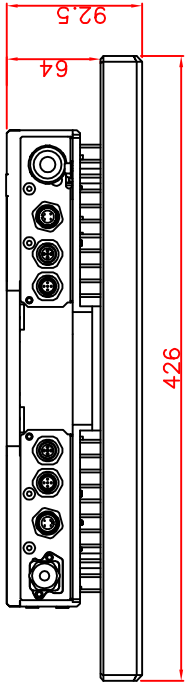
bottom view
