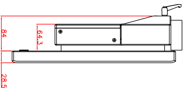
left view
