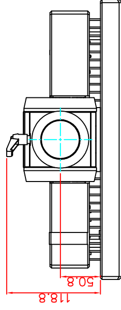
bottom view
