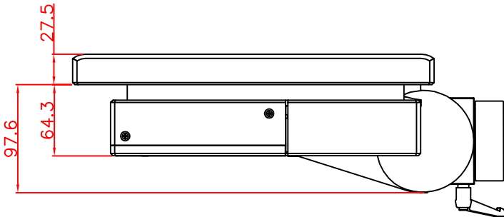
left view
