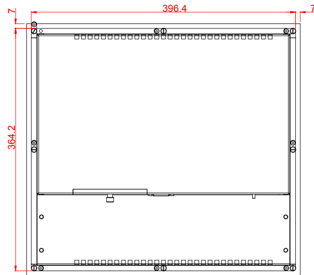
rear view
