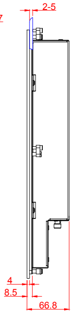
left view
