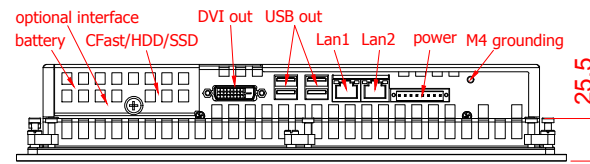
bottom view
