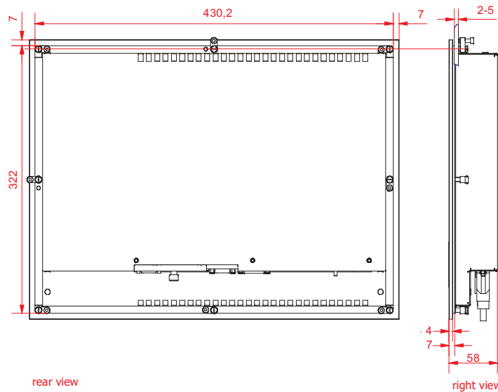
right view
