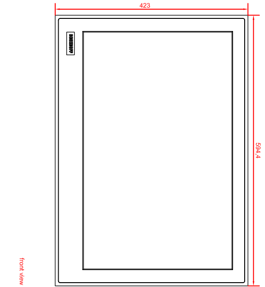
CP6204-0001-0030 main dimensions
