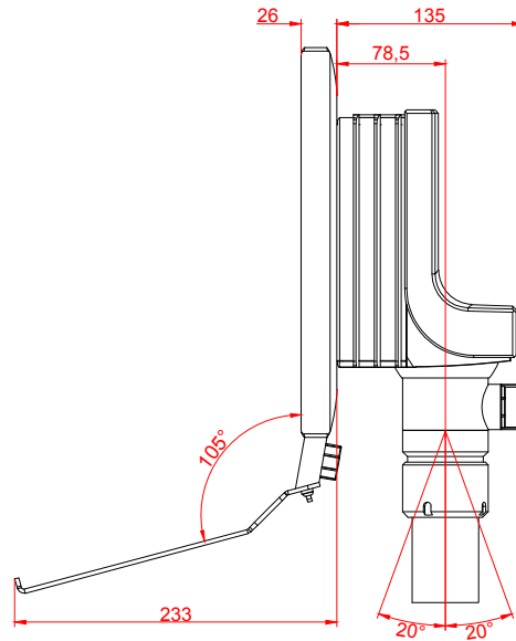
right view
