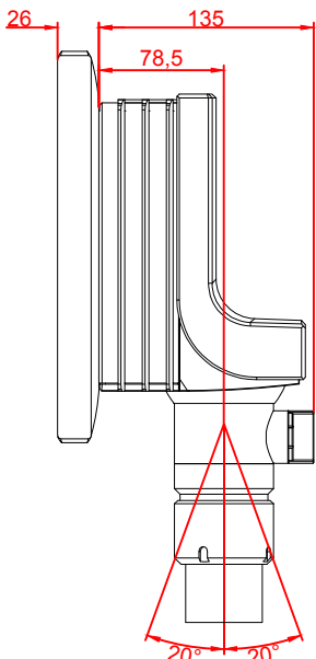
left view
