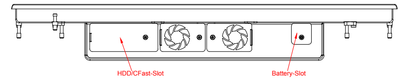
top view
