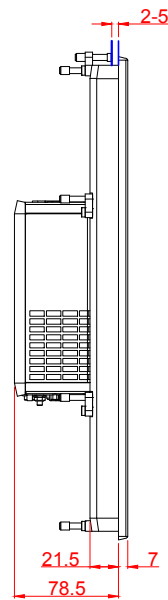
left view
