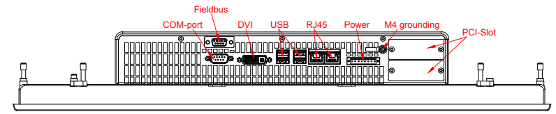
bottom view
