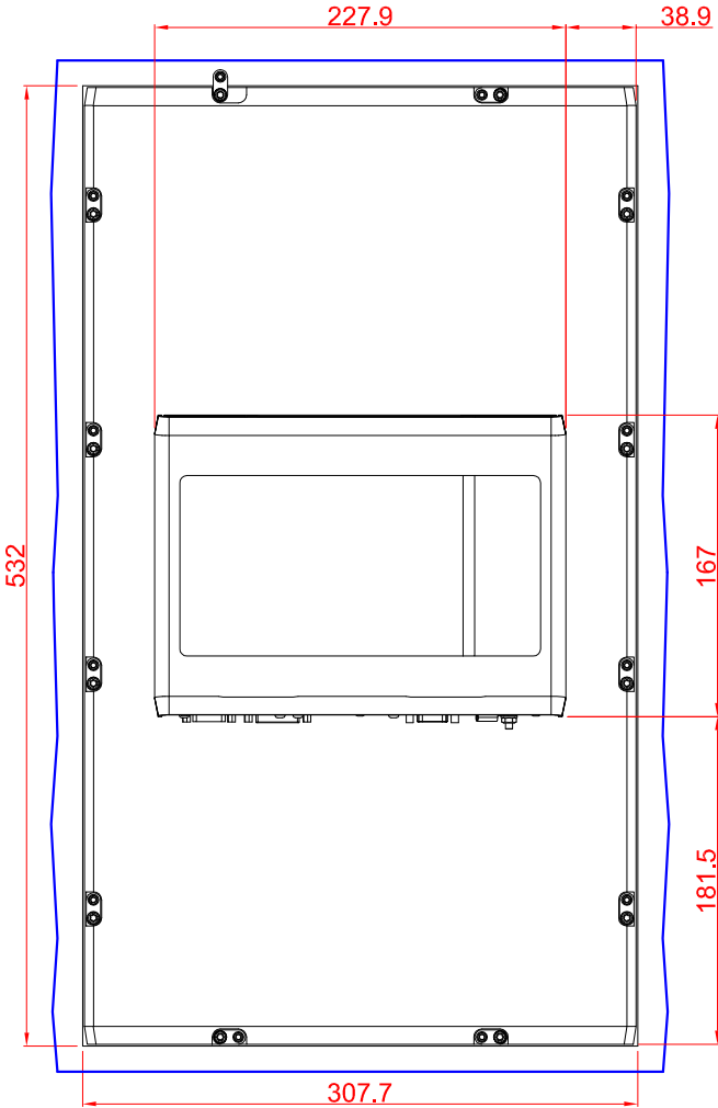
bottom view
