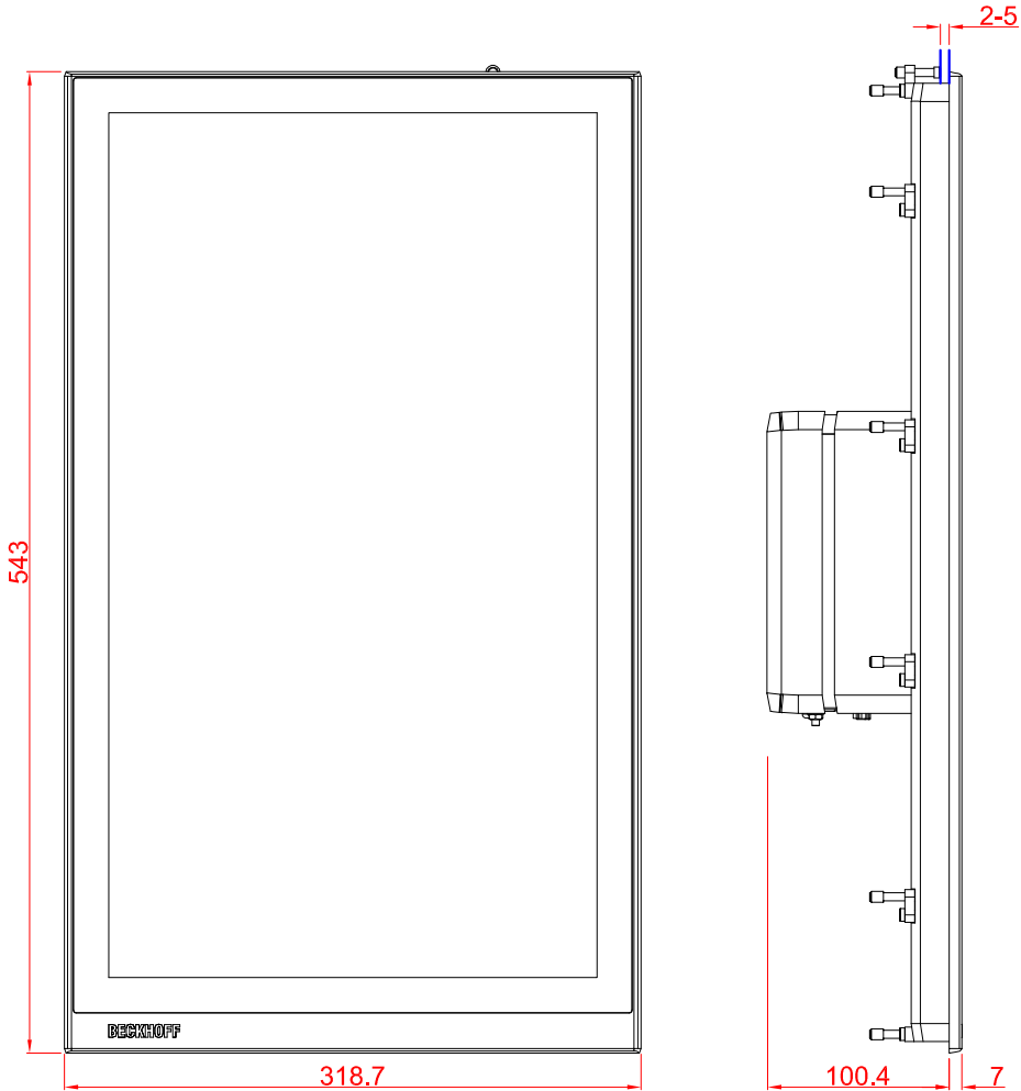
front view
