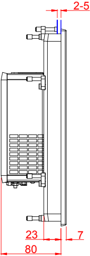
left view
