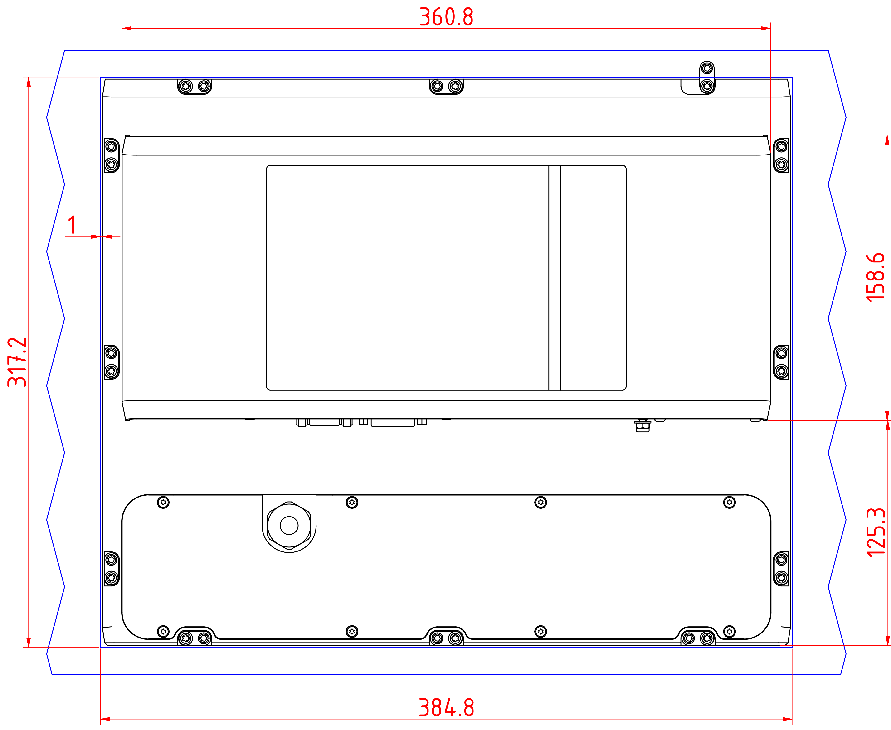
cut out dimensions: 317.2mm x384.8mm rear view
