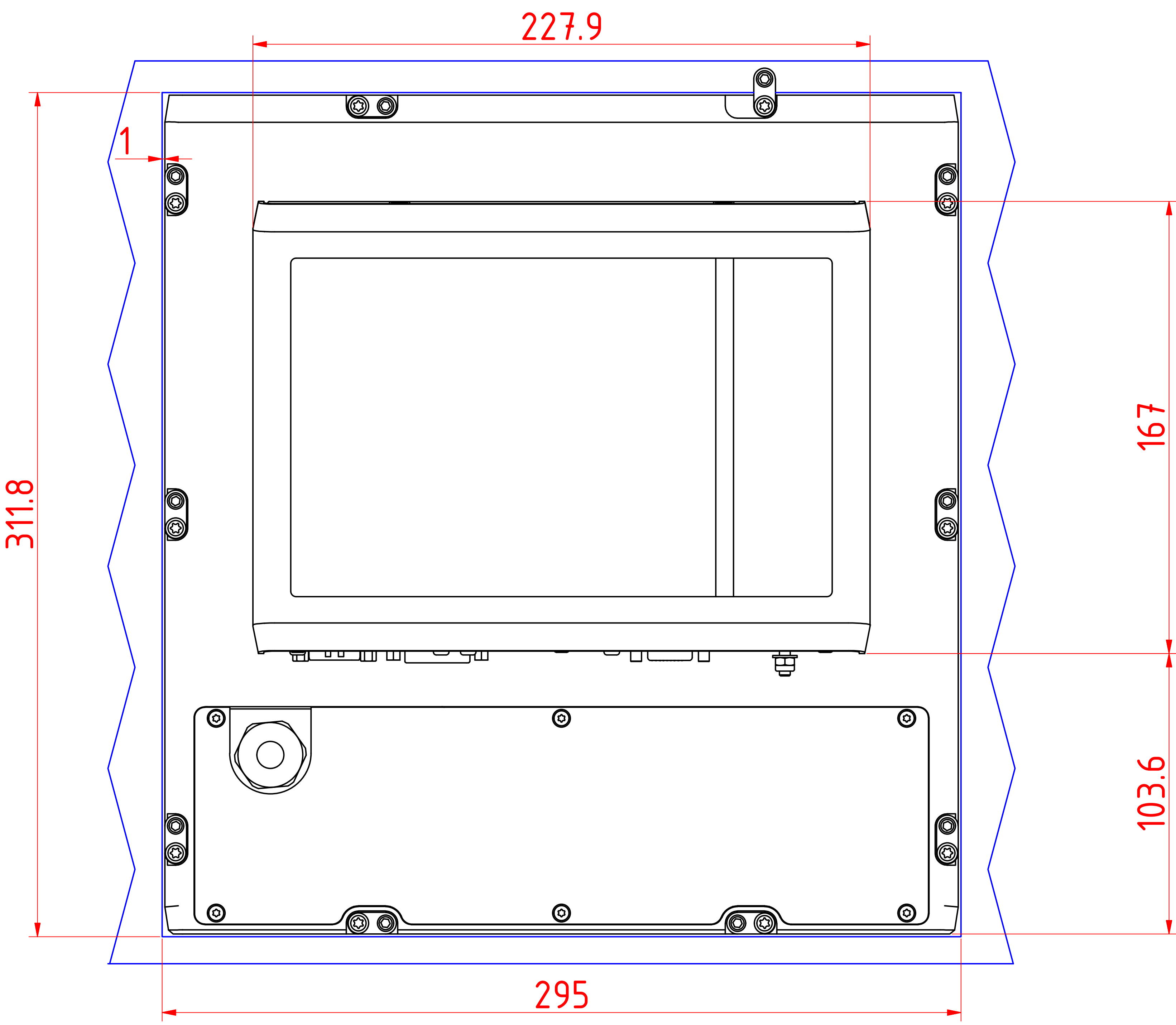
cut out dimensions: 311.8mm x 295mm rear view
