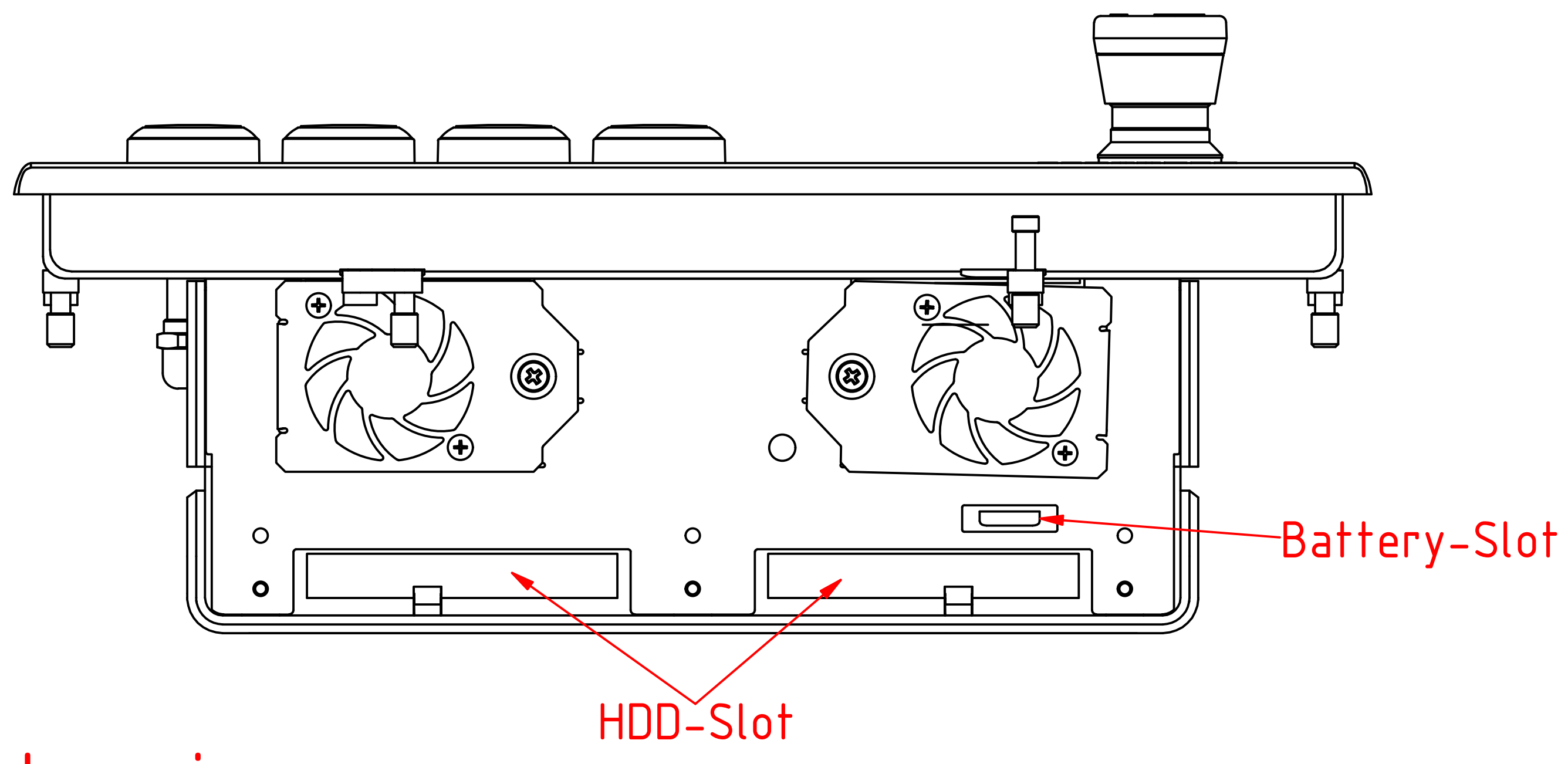
top view
