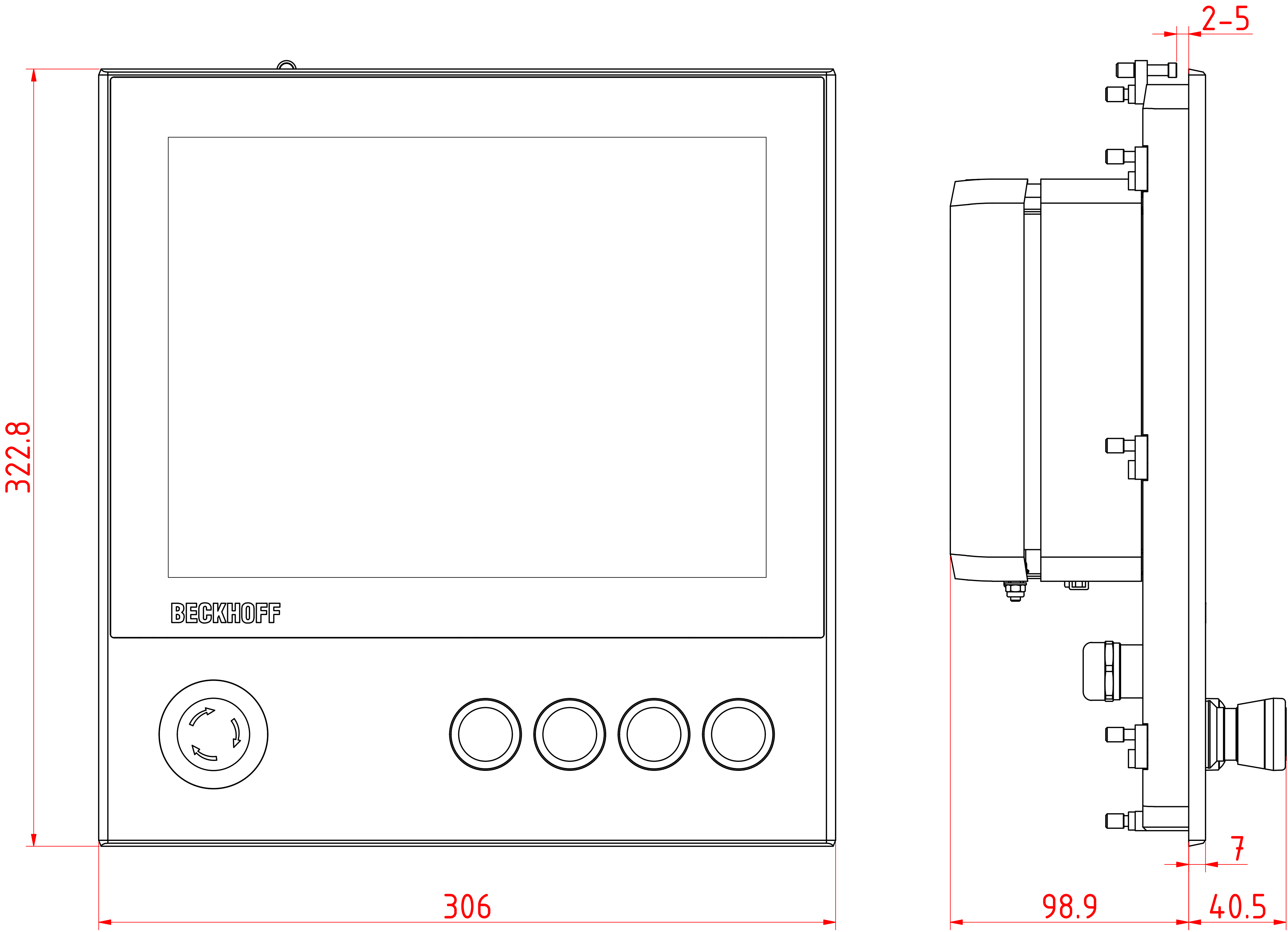
front view
