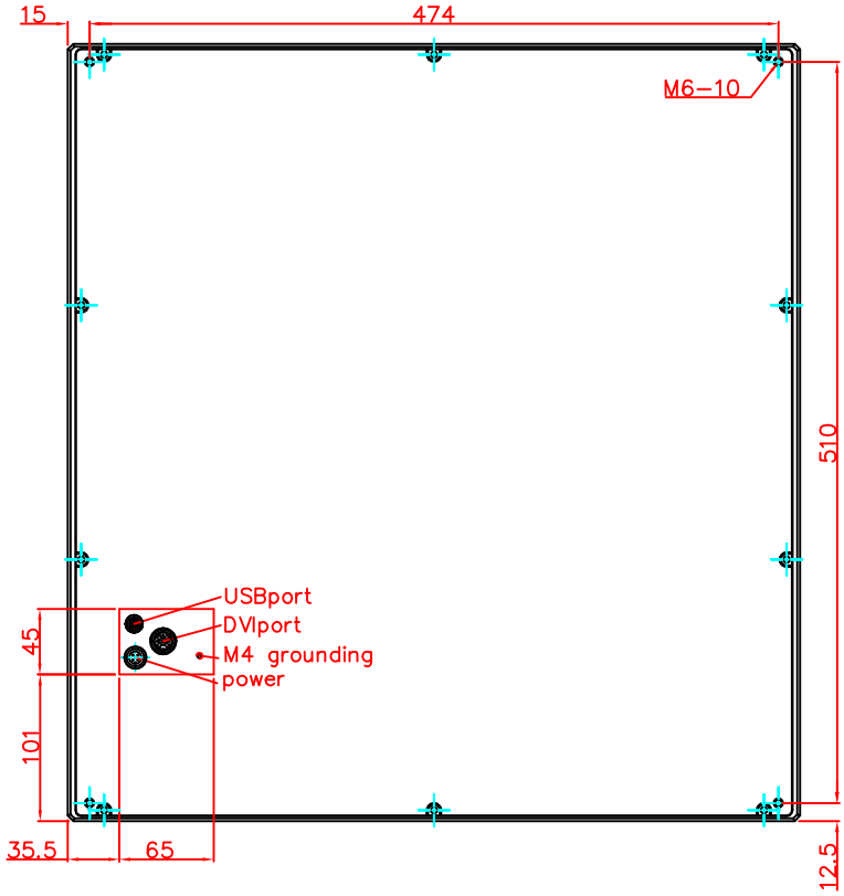
rear view
