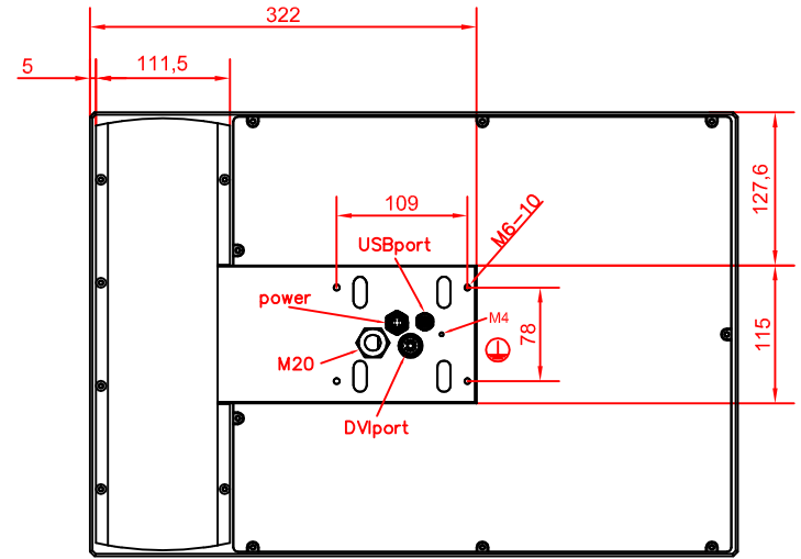
rear view
