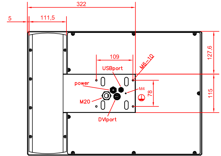
rear view
