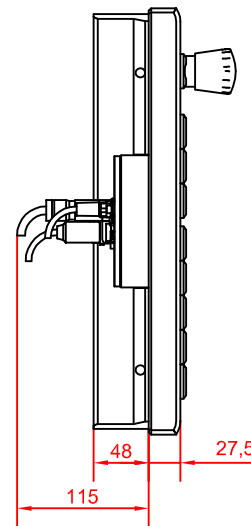
left view
