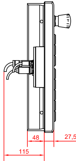
left view
