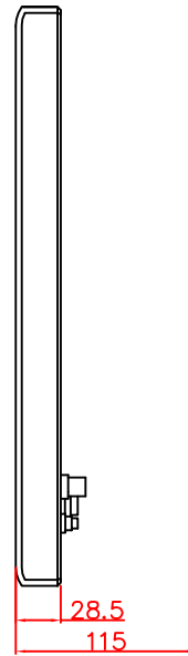
right view
