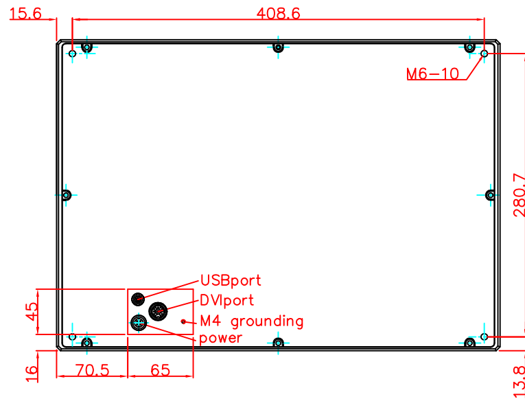
rear view
