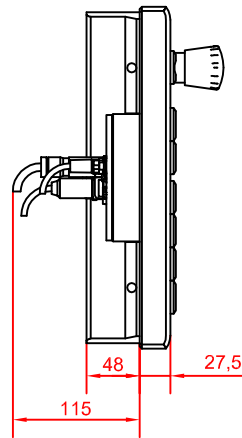
left view
