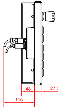
left view
