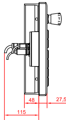
left view
