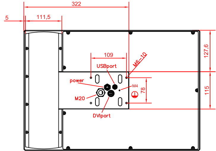
rear view
