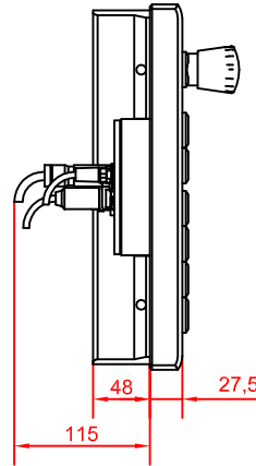
left view
