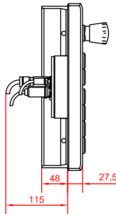
left view
