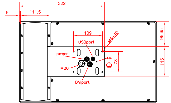
rear view
