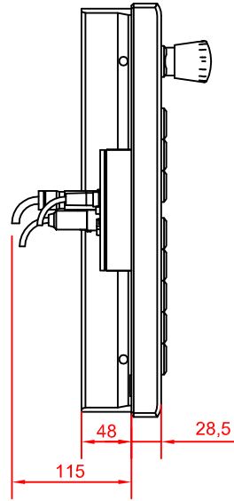
left view
