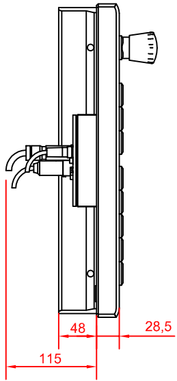
left view
