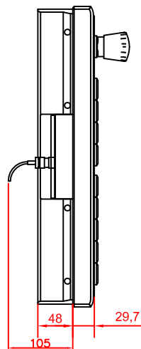
left view
