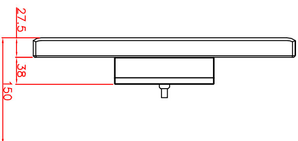
right view
