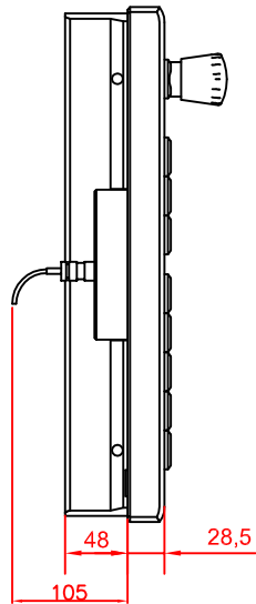
left view
