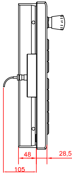
left view
