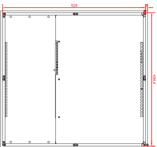
rear view dimensions in mm
