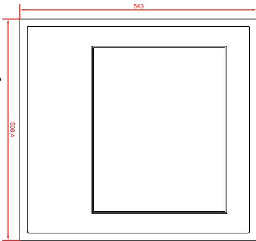
CP6833-0001 main dimensions
