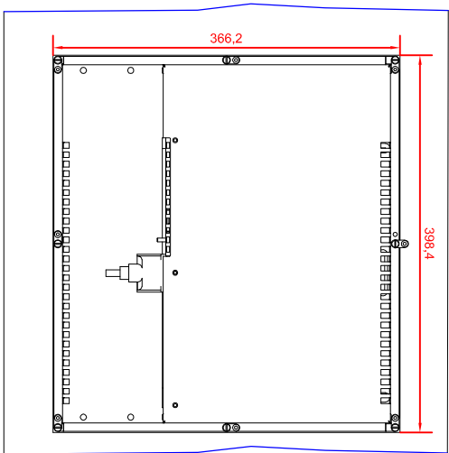
rear view width install measure
