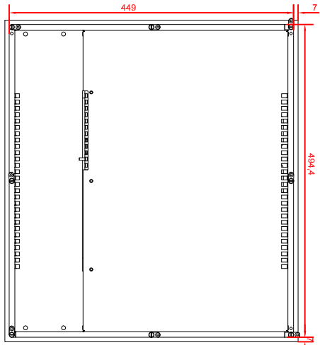
rear view dimensions in mm
