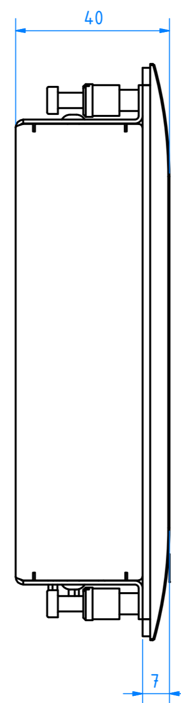
left view
