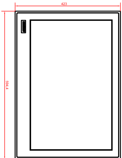
CP6904-0000 main dimensions
