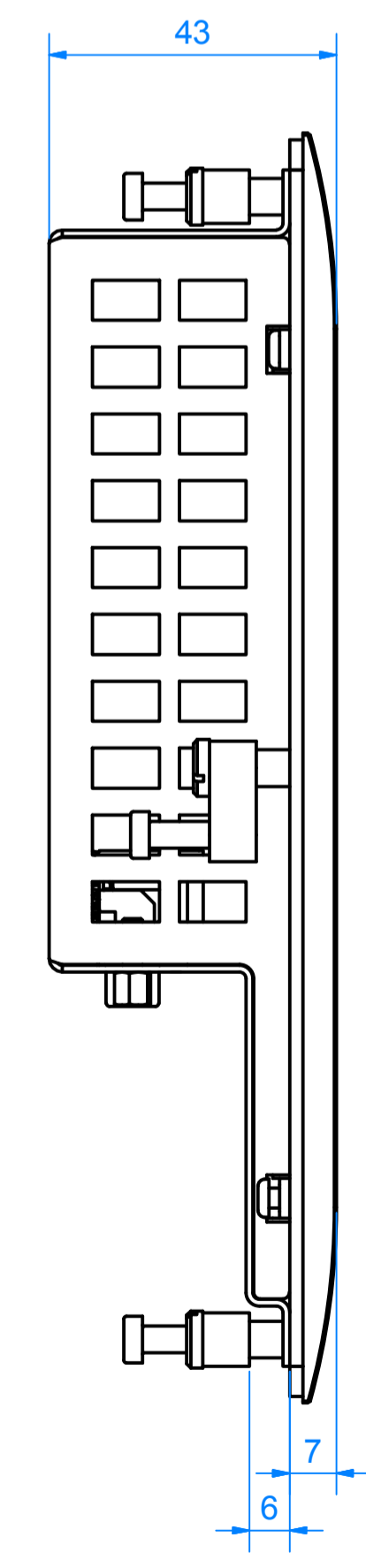
left view
