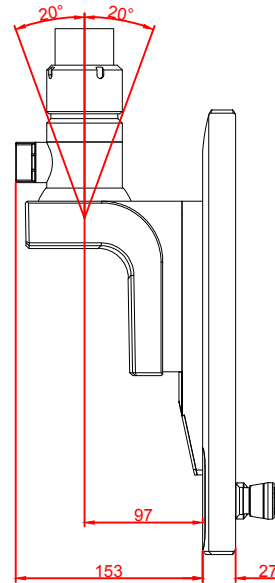
left view
