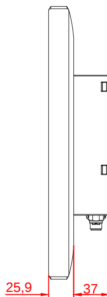
left view
