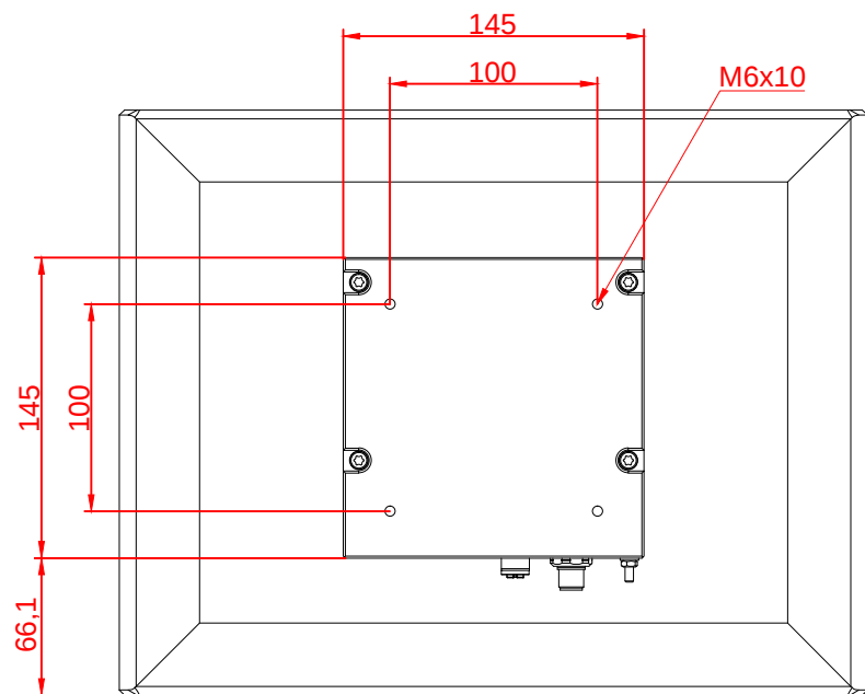
rear view
