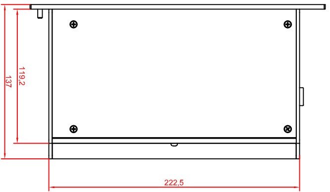
left view
