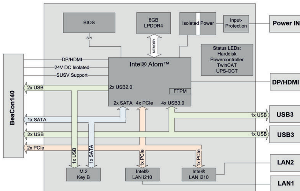
Fig. 1: CB6273 Block diagram
