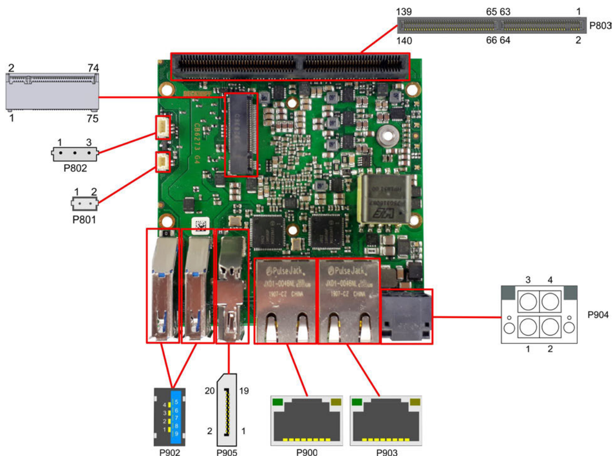
Fig. 2: CB6273 Plug connections overview
