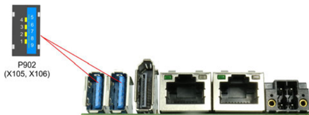
Fig. 6: CB6273 Frontpanel USB
