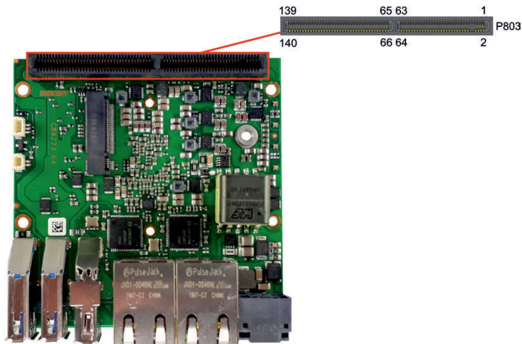
Fig. 7: CB6273 BeaCon140-G4
