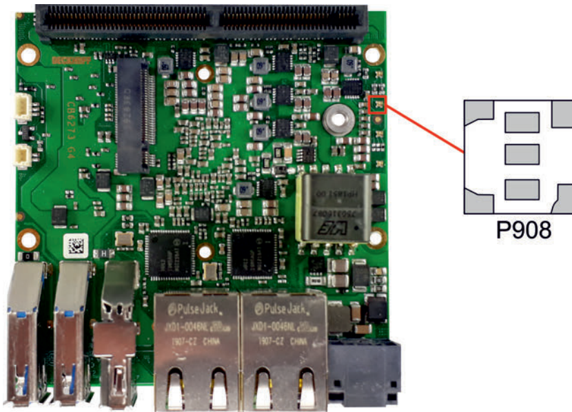
Fig. 13: CB6273 TwinCAT-LED
