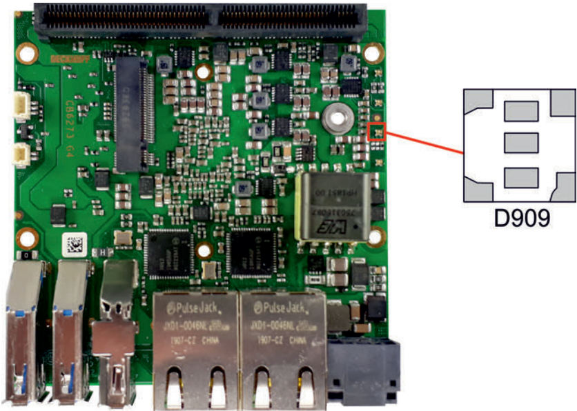
Fig. 12: CB6273 SATA-LED
