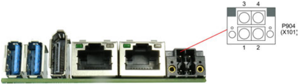
Fig. 3: CB6273 Frontpanel Power
